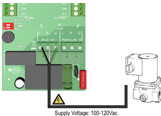
Gas Supply Controlled by 100-120VAC Solenoid Valve
