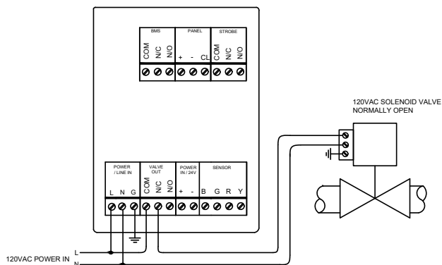
120VAC SOLENOID VALVE NORMALLY OPEN
