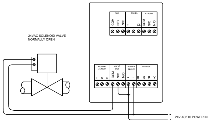
24VAC SOLENOID VALVE NORMALLY OPEN
