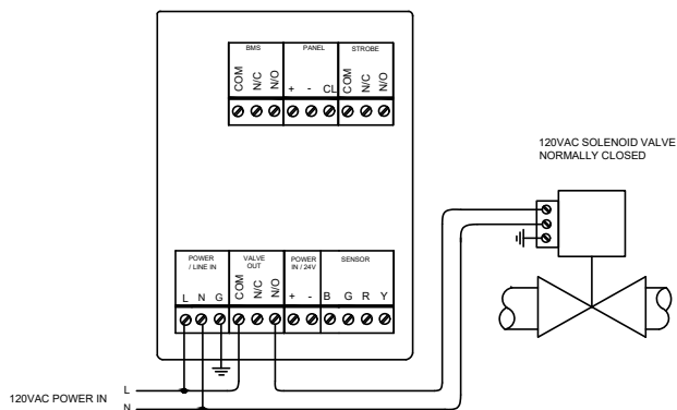
120VAC SOLENOID VALVE NORMALLY CLOSED
