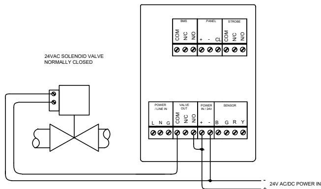
24VAC SOLENOID VALVE NORMALLY CLOSED
